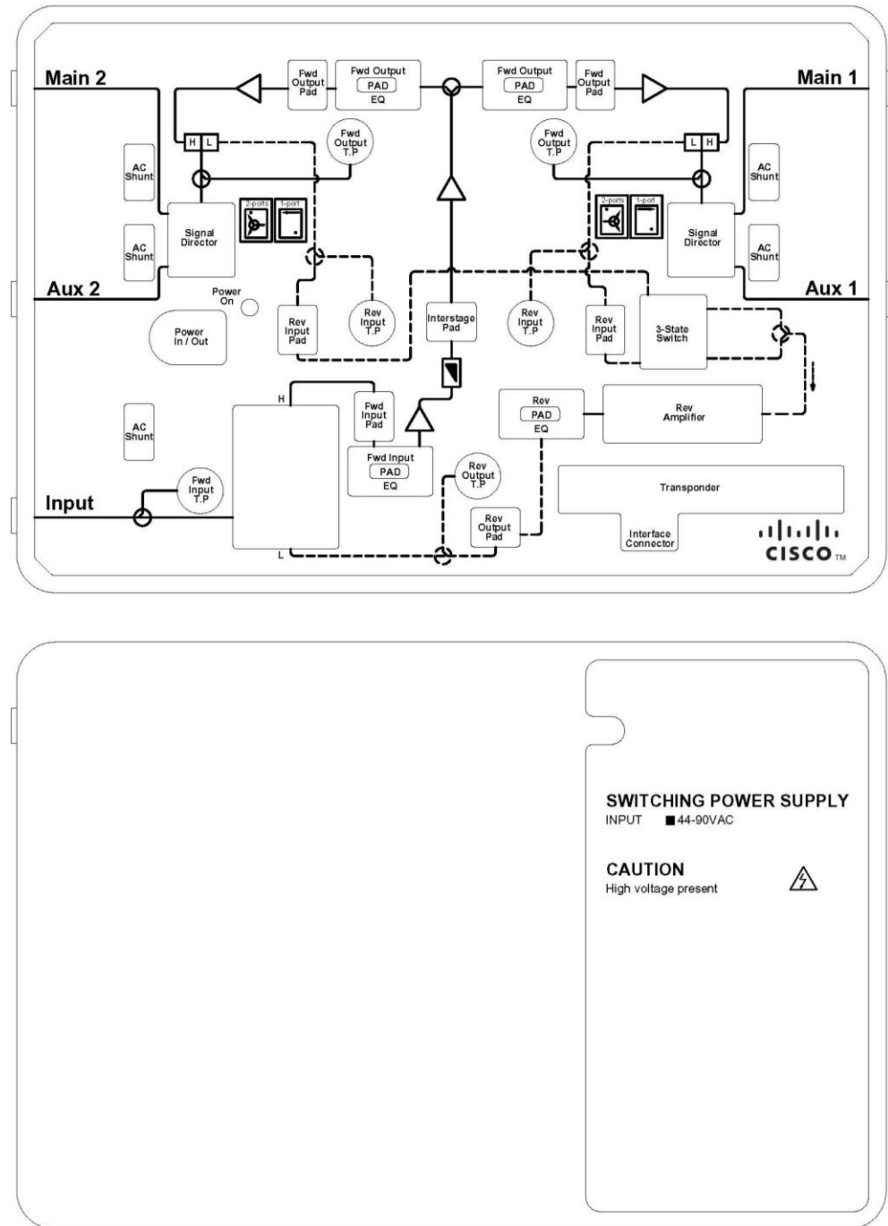
Figure 3. Block Diagram
